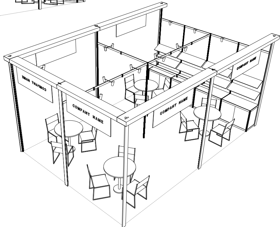
PERSPECTIVE VIEW
